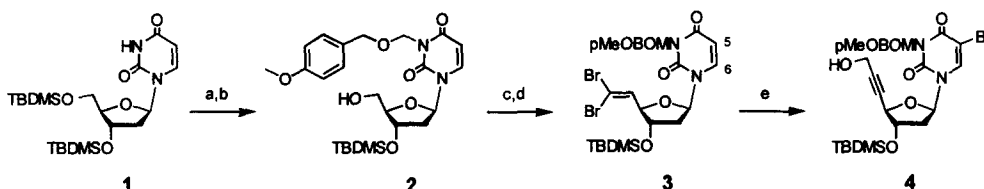
Scheme 1. a) pMeOBOMCl (1.6 eq.), DBU (4.1 eq.), \text{CH}_3\text{CN} , 0^\circ\text{C} , 2h30, 96%. b) TFA (1.7 eq.), \text{THF}/\text{H}_2\text{O} 3/1, rt, 9h30, 61%. c) Oxalyl chloride (1.6 eq.), DMSO (3.1 eq.), \text{CH}_2\text{Cl}_2 , -78^\circ\text{C} , 1h30. d) \text{NEt}_3 (6.3 eq.), \text{Ph}_3\text{P}=\text{CBr}_2 (2.0 eq.), 0^\circ\text{C} to rt, 24h. e) LDA (2.1 eq.), THF, -78^\circ\text{C} , 30min then (\text{CH}_2\text{O})_n (excess), 0^\circ\text{C} to rt, 2h, 52%.
