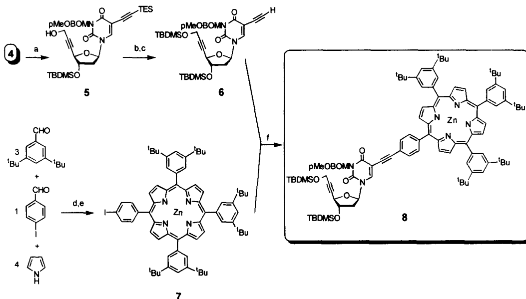
Scheme 2. a) HCCTES (3.9 eq.), CuI (0.60 eq.), Pd(PPh 3 ) 2 Cl 2 (0.24 eq.), NEt 3 , rt, 24h, 86%. b) TBDMSCl (1.3 eq.), imidazole (3.2 eq.), DMF, rt, 18h, 89%. c) K 2 CO 3 (4.6 eq.), THF/MeOH 1/1, 3h30 at 0°C and 4h at 10°C, 77%. d) BF 3 ·OEt 2 (1.9 eq.), CHCl 3 , rt, 1h then chloranil (3.0 eq.), CHCl 3 , reflux, 1h, 5%. e) Zn(OAc) 2 ·2H 2 O (1.9 eq.), CHCl 3 , reflux, 1h30, 91%. f) CuI (0.86 eq.), Pd(PPh 3 ) 2 Cl 2 (0.47 eq.), NEt 3 , rt, 24h, 40%.
