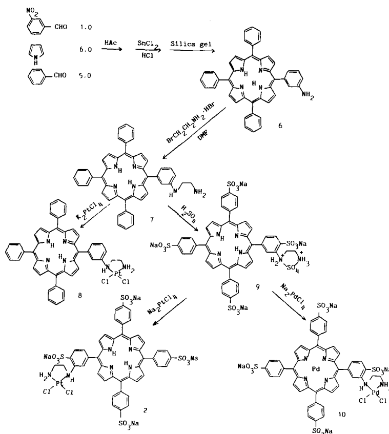
Scheme II Reaction Route for the Synthesis of Mono-( m -NH 2 CH 2 CH 2 NH 2 )-TPPS 4 and Its Pt(II) and Pd(II) Complexes
