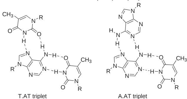
Natural nucleobase-triplets (examples):
