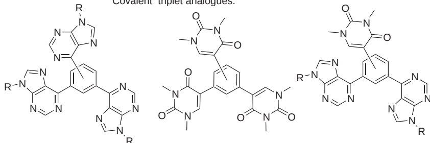
Covalent triplet analogues:
