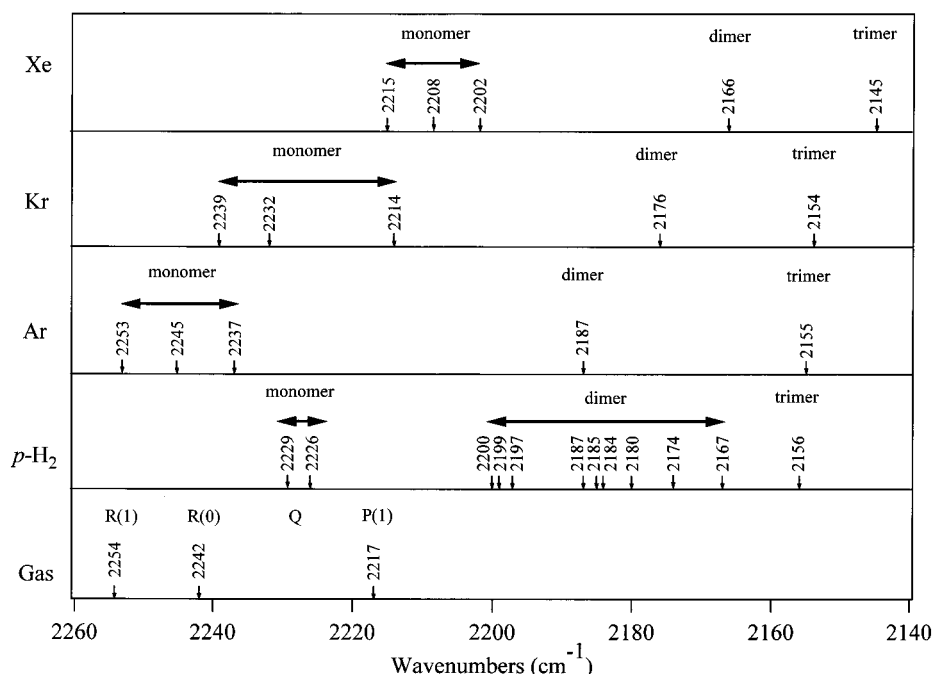
Figure 2. Collection of the spectral information on the HI stretching vibration for monomer, dimers, and trimers. The references for Xe, Kr, and Ar matrixes are refs 12, 13, and 14, respectively. The stick spectrum for p\text{-H}_2 is constructed by reproducing the major observed peaks in Figure 1a. The frequencies of gaseous HI were measured at room temperatures with the spectrometer described in the Experimental Section.
