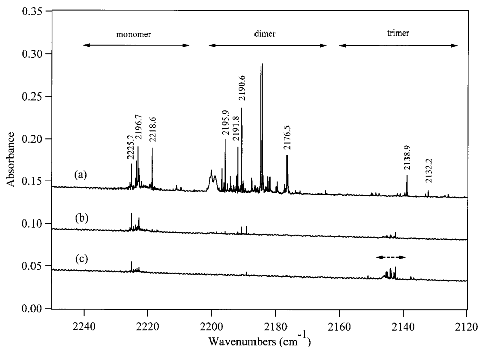
Figure 3. FTIR spectra in the HI stretching region of sample in solid parahydrogen with a composition of CO 2 /HI/ p -H 2 = 15:1:2 × 10 6 : (a) the sample immediately after the deposition; (b) same as (a) after an initial 180 min UV irradiation; (c) same as (b) after an additional 240 min irradiation followed by a dark period of 300 min and a further irradiation for 240 min. Thus, the total irradiation time amounts to 180 + 240 × 2 = 660 min. The peaks shown with frequencies appear newly contrary to the case of Figure 1a. The dashed-line arrow in (c) shows the CO stretching vibration. The multiple peaks may reflect the subtle difference of the environment of CO.
