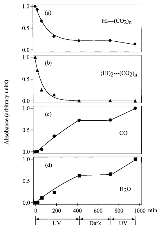
Figure 4. The upper two panels show the temporal change of the integrated intensities of the HI stretching vibration for monomeric HI and (\text{HI})_2 complexed with small \text{CO}_2 clusters. The plots are obtained by the integration of peaks under the arrows of “monomer” and “dimer” spectral regions in Figure 3. The lower two panels are obtained by plotting the integrated intensity of the CO stretching vibration in Figure 3c and the intensity of the antisymmetric stretching vibration of \text{H}_2\text{O} shown in the right-hand-side of Figure 6, respectively. The horizontal portions in the eye-guide curves denoted by “Dark” corresponds to a 300 min dark period at 4.9 K. Except for this period, the abscissa is for the UV irradiation time.
