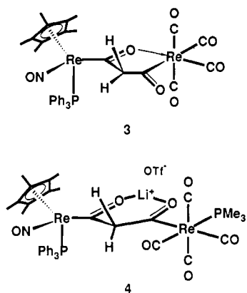
Figure 1. Molecular structure of 4 showing orientation of \text{CF}_3\text{SO}_3^- and \text{Li}^+ ions in relation to the dirhenium backbone. Bond distances (Å) and angles (deg) are as follows: \text{Re}(1)\text{--C}(42) 2.069 (9), \text{Re}(2)\text{--P}(2) 2.453 (5), \text{Re}(2)\text{--C}(44) 2.194 (11), \text{C}(42)\text{--C}(43) 1.563 (16), \text{C}(43)\text{--C}(44) 1.516 (16), \text{C}(42)\text{--O}(42) 1.228 (12), \text{C}(44)\text{--O}(44) 1.254 (13), \text{C}(43)\text{--H(a)} 0.935 (98), \text{C}(43)\text{--H(b)} 0.939 (148); \text{C}(42)\text{--C}(43)\text{--C}(44) 116.5 (9), \text{Re}(1)\text{--C}(42)\text{--C}(43) 120.5 (7), \text{Re}(2)\text{--C}(44)\text{--C}(43) 123.6 (7), \text{Re}(1)\text{--C}(42)\text{--O}(42) 124.9 (8), \text{Re}(2)\text{--C}(44)\text{--O}(44) 119.9 (8), \text{C}(43)\text{--C}(42)\text{--O}(42) 114.6 (8), \text{C}(43)\text{--C}(44)\text{--O}(44) 116.4 (9), \text{C}(42)\text{--Re}(1)\text{--P}(2) 86.6 (3), \text{C}(44)\text{--Re}(2)\text{--P}(2) 84.3 (3), \text{Li--O}(42) 1.940, \text{Li--O}(44) 1.908, \text{Li--O}(3) 1.922, \text{Li--O}(2a) 1.902 Å; the average \text{O--Li--O} angle is 109.1.
