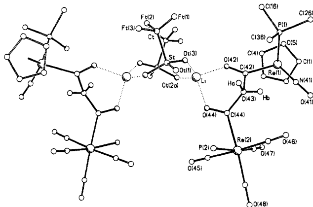
Figure 1. Molecular structure of 4 showing orientation of \text{CF}_3\text{SO}_3^- and \text{Li}^+ ions in relation to the dirhenium backbone. Bond distances (Å) and angles (deg) are as follows: \text{Re}(1)\text{--C}(42) 2.069 (9), \text{Re}(2)\text{--P}(2) 2.453 (5), \text{Re}(2)\text{--C}(44) 2.194 (11), \text{C}(42)\text{--C}(43) 1.563 (16), \text{C}(43)\text{--C}(44) 1.516 (16), \text{C}(42)\text{--O}(42) 1.228 (12), \text{C}(44)\text{--O}(44) 1.254 (13), \text{C}(43)\text{--H(a)} 0.935 (98), \text{C}(43)\text{--H(b)} 0.939 (148); \text{C}(42)\text{--C}(43)\text{--C}(44) 116.5 (9), \text{Re}(1)\text{--C}(42)\text{--C}(43) 120.5 (7), \text{Re}(2)\text{--C}(44)\text{--C}(43) 123.6 (7), \text{Re}(1)\text{--C}(42)\text{--O}(42) 124.9 (8), \text{Re}(2)\text{--C}(44)\text{--O}(44) 119.9 (8), \text{C}(43)\text{--C}(42)\text{--O}(42) 114.6 (8), \text{C}(43)\text{--C}(44)\text{--O}(44) 116.4 (9), \text{C}(42)\text{--Re}(1)\text{--P}(2) 86.6 (3), \text{C}(44)\text{--Re}(2)\text{--P}(2) 84.3 (3), \text{Li--O}(42) 1.940, \text{Li--O}(44) 1.908, \text{Li--O}(3) 1.922, \text{Li--O}(2a) 1.902 Å; the average \text{O--Li--O} angle is 109.1.
