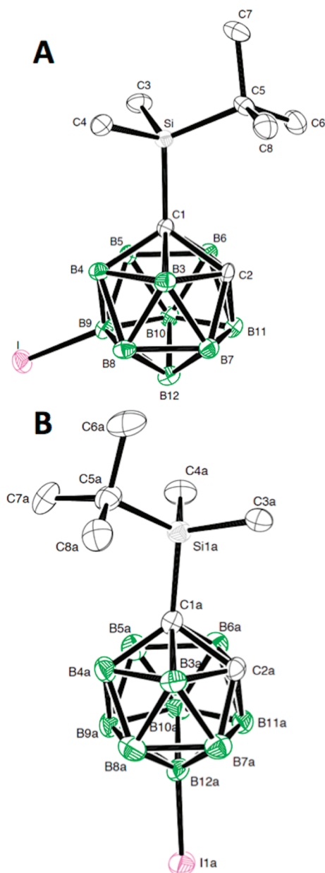
Figure 4. ORTEP plots of 8a and 8b drawn with 50% probability displacement ellipsoids. The hydrogen atoms are omitted for clarity. Only one of the four molecules in the asymmetric unit, molecule A , is shown for structure 8b .
