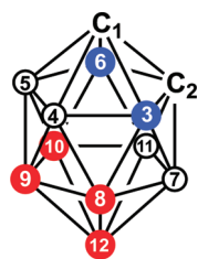
Figure 2. Atom numbering and electron density distribution in closo-o -carborane. Boron atoms shown in red are the most electron-rich, whereas the boron atoms shown in blue are the most electron-deficient.
