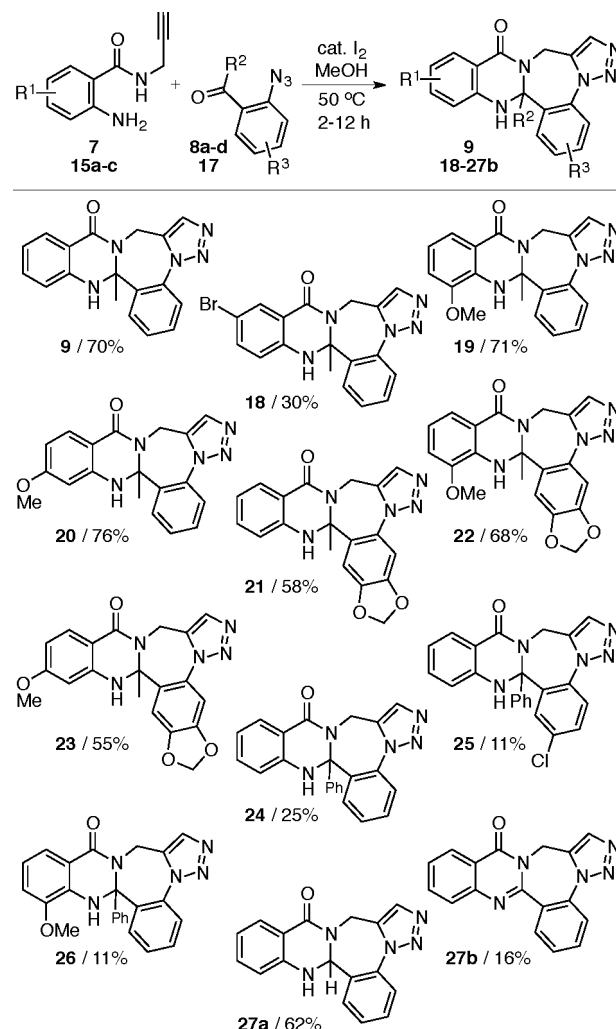
Figure 2. Substrate scope; isolated yields shown. Note: all products were characterized by ^1\text{H} and ^{13}\text{C} NMR, IR, and HRMS.
