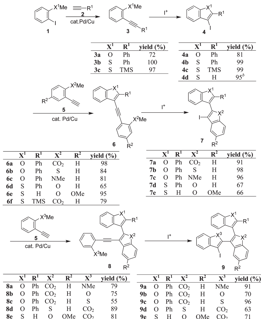
SCHEME 2. Generation of Polyheterocyclic Compounds by the General Strategy a
