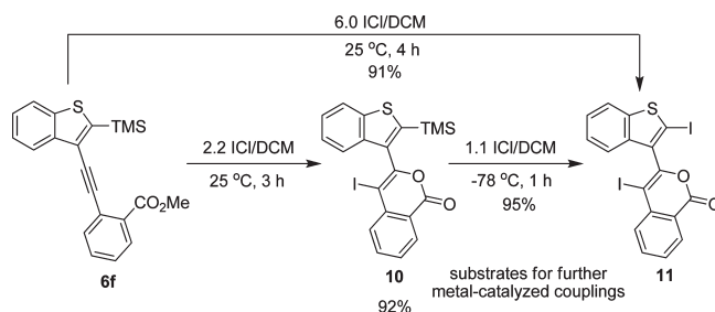
SCHEME 3. Simultaneous and Stepwise Diiodination
