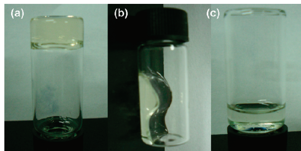
Figure 2. State changes during the melting process of the gel 1 (0.7 g/100 cm 3 ) in 1,2-dichloroethane: (a) gel obtained at 20 °C; (b) gel–sol phase at 42 °C; (c) solution above 42 °C (the T_{\text{gel}} of 1 in 1,2-dichloroethane).
