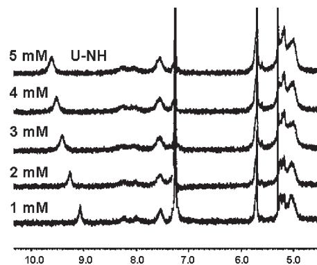
Figure 5. Partial ^1\text{H} NMR spectra (300 MHz, \text{CDCl}_3 ) of 1 at different concentrations at 25 °C.
