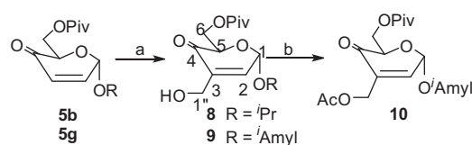
Scheme 3. Reagents and conditions: (a) 37% aq. \text{HCHO} , DMAP, THF, -5^\circ\text{C} , 12 h–16 h; (b) (\text{CH}_3\text{CO})_2\text{O} , Pyridine, 0^\circ\text{C} \rightarrow 5^\circ\text{C} , 12 h.
