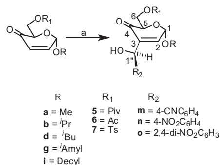
Scheme 2. Reagents and conditions: (a) \text{TiCl}_4 , TBAI, \text{R}_2\text{CHO} , DCM, 5 h–8 h, -78^\circ\text{C} \rightarrow -30^\circ\text{C} .
