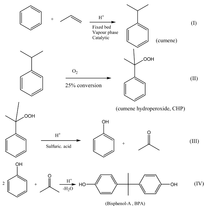
Scheme 1. Hock process of phenol manufacture (steps I–III) and BPA manufacture from phenol and acetone (step IV)
