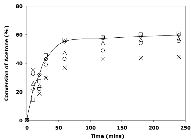
Figure 2. Effect of speed of agitation. Reaction conditions: mole ratio of CHP/phenol = 1:5; temperature: 100 °C; catalyst loading: 0.025 g/cm 3 .
