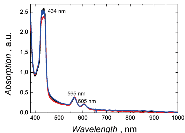
Figure 10. UV/vis absorption spectra of ZnO mesoporous films functionalized with 18 (red line), 19 (black line), and 20 (blue line) after sensitization with 21 .
