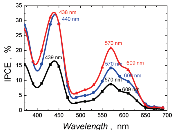
Figure 12. IPCE spectra of differently functionalized ZnO films sensitized with porphyrin, for ZnO electrodes grafted with 18 (red line), 19 (black line), and 20 (blue line) before dye sensitization.
