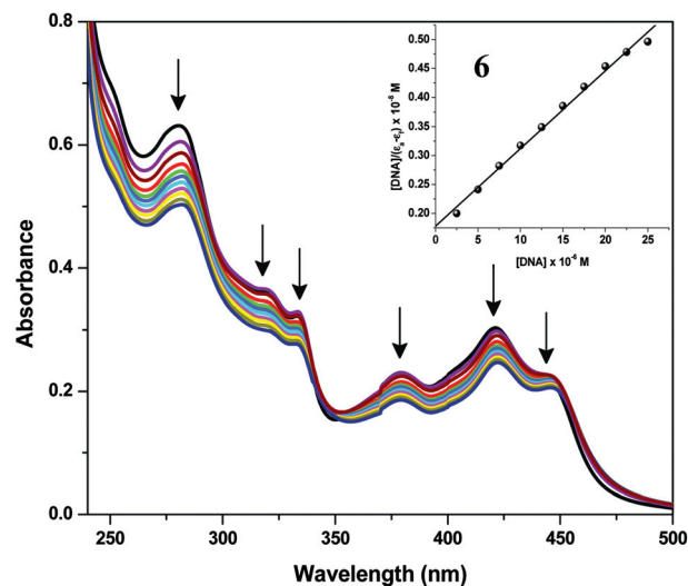
Fig. 3 Electronic absorption spectra of complex 6 (25 \mu\text{M} ) in the absence and presence of increasing amounts of CT DNA (2.5, 5.0, 7.5, 10.0, 12.5, 15.0, 17.5 and 20.0, 22.5 and 25 \mu\text{M} ). Arrows show the changes in absorbance as a function of increasing DNA concentration (inset: plot of [\text{DNA}] vs. [\text{DNA}]/(\epsilon_a - \epsilon_f) ).
