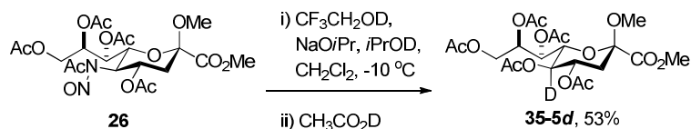
Scheme 5. Deuterium Incorporation at the 5-Position of KDN.
