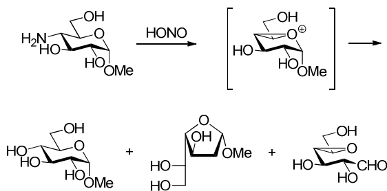
Scheme 8. Deamination Reactions in the 4-Amino-4-deoxyglucose Series
