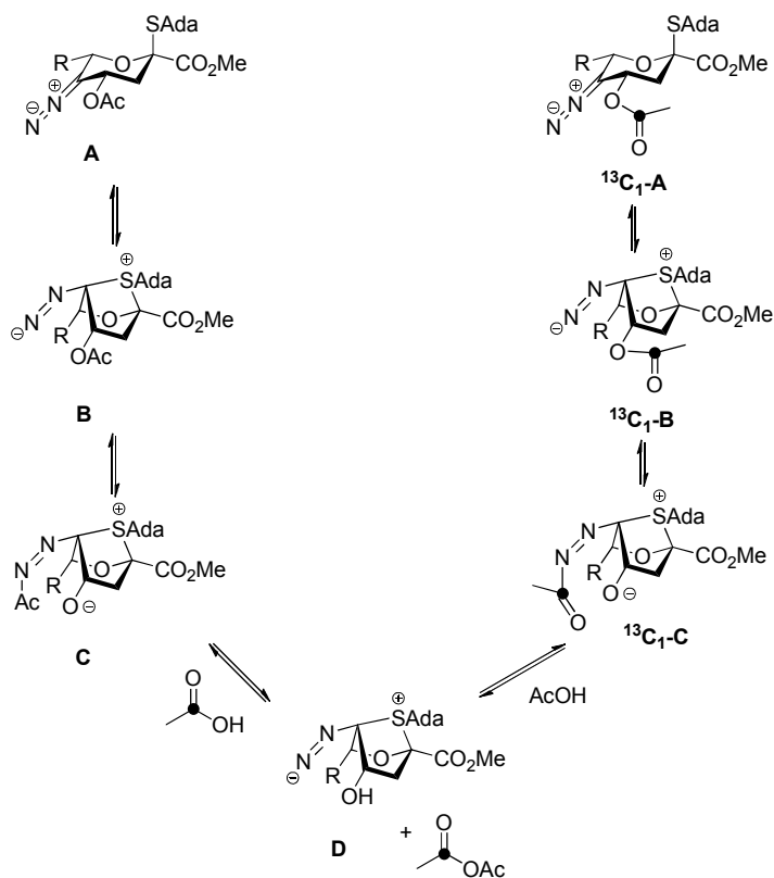
Scheme 12. Incorporation of ^{13}\text{C} -Labelled Acetate at O4 in the Axial Thioglycoside 53 .
