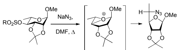
Scheme 9. Ring Contraction of a Rhamnosyl 4- O -Sulfonate
