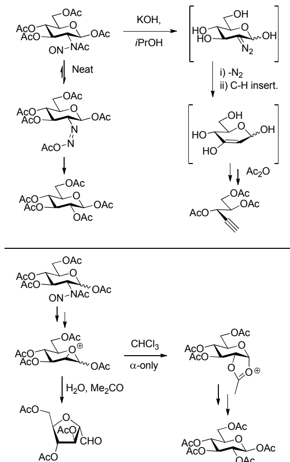
Scheme 10. Deamination Reactions in the Glucosamine Series
