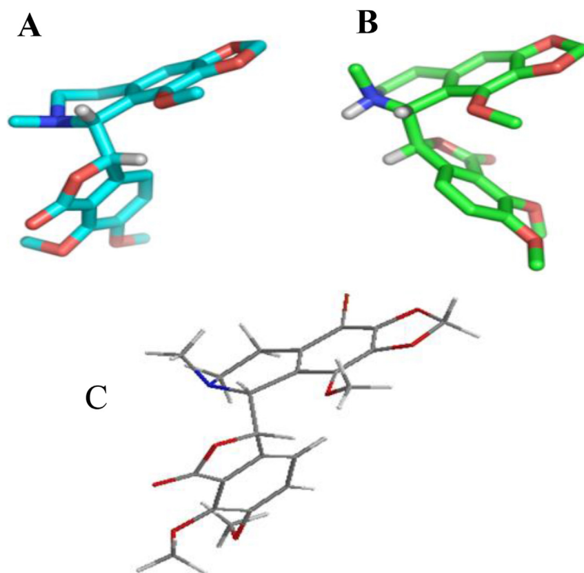
Fig. 3. The X-ray crystal structures of natural noscapine free base ( 1 , Panel A), its HCl salt (Panel B) and 9'-bromonoscapine ( 2 , Panel C).
