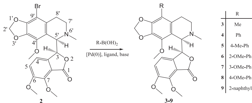
Scheme 1. Synthesis of targeted 9'-alkyl- and arylnoscapines 3–9 .
