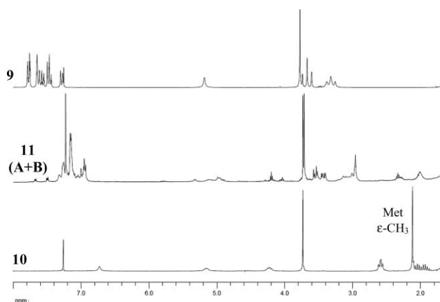
Fig. 8 400 MHz ^1\text{H} NMR spectra in \text{CDCl}_3 solution of Boc-( S )-BpAib-OMe 9 , Boc-( S )-Met-Aib-OMe 10 , and the mixture of the two diastereomeric products ( 11A and 11B ) isolated after the photoreaction.
