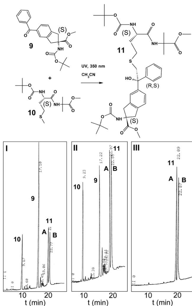
Fig. 7 Top: chemical structures of the Boc-( S )-BpAib-OMe 9 and Boc-( S )-Met-Aib-OMe 10 reagents and the products ( 11 ) of the photoreaction; bottom: reverse-phase HPLC profiles of the photoreaction mixture after 25 min ( I ) and 60 min ( II ). Part III shows the HPLC profile of the two photoreaction products after a flash chromatography purification of the crude mixture.
