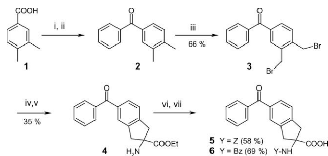
Fig. 2 Synthesis of N ^{\alpha} -protected (blocked) BpAib. (i) SOCl 2 ; DMF; rt. (ii) AlCl 3 , benzene; DCE; rt. (iii) NBS, benzoyl peroxide; CCl 4 ; 90 °C. (iv) NC–CH 2 –COOEt; K 2 CO 3 ; n Bu 4 N + ·HSO 4 – (cat.); CH 3 CN; 80 °C. (v) 10 N aq. HCl; abs. EtOH; 0 °C to rt. (vi) Z-OSu or (Bz) 2 O; CH 3 CN; rt. (vii) NaOH; MeOH–THF–H 2 O; 60 °C.
