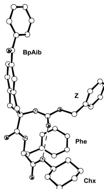
Fig. 4 X-Ray diffraction structure of the N ^{\alpha} -protected dipeptide alkylamide Z-( R )-BpAib-( S )-Phe-NHChx 8a . The intramolecular C=O...H–N H-bond is represented by a dashed line.
