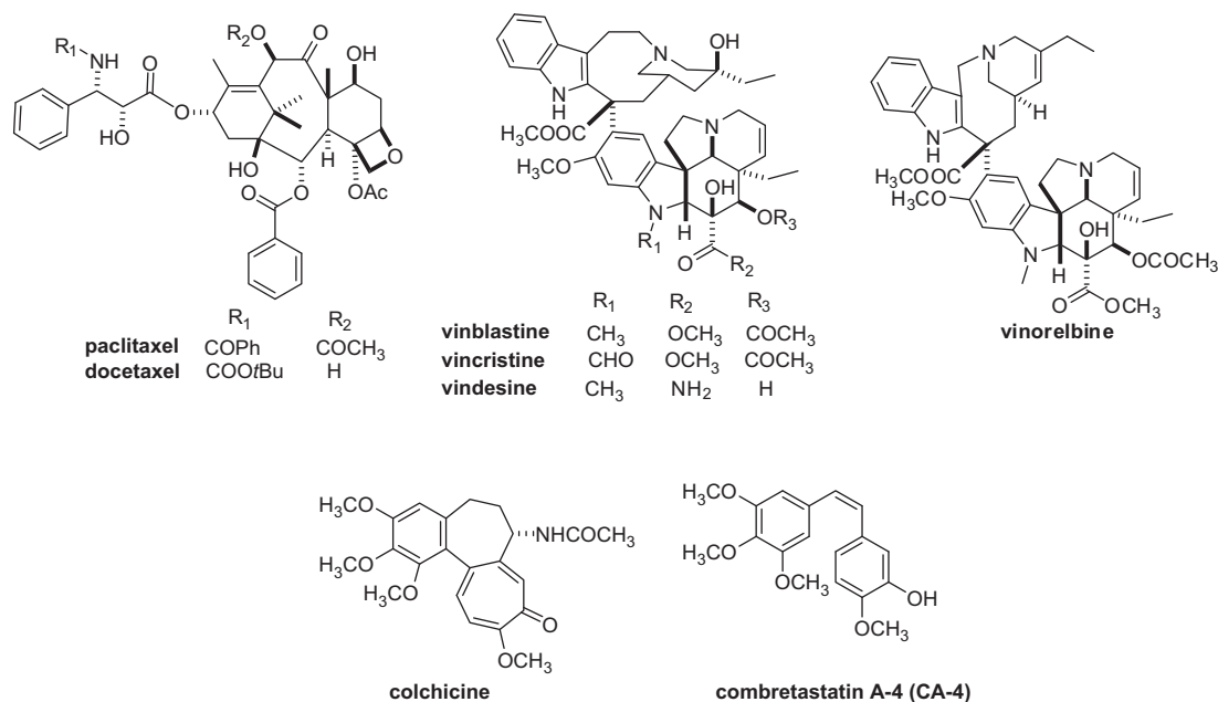
Figure 1. Tubulin binding agents.
