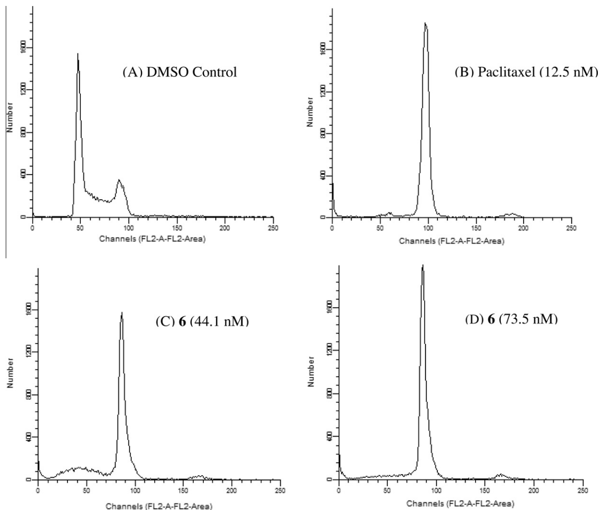
Figure 4. The effects of 6 on cell cycle distribution. MDA-MD-435 cells were treated with vehicle (A), 12.5 nM paclitaxel ( 6.5 \times IC_{50} for inhibition of proliferation) (B), 44.1 nM 6 ( 3 \times IC_{50} ) (C), or 73.5 nM 6 ( 5 \times IC_{50} ) (D), for 18 h. The cells were harvested and stained with propidium iodide, and cell cycle distribution was evaluated using flow cytometry.
