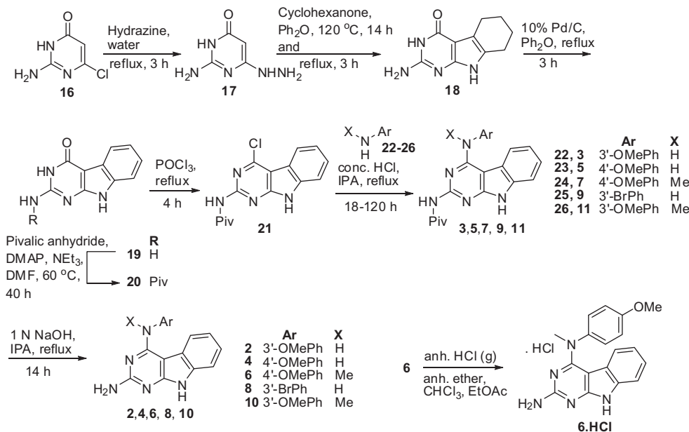
Scheme 1. Synthesis of compounds 2–11 and 6.HCl.
