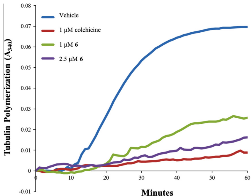
Figure 5. Effects of 6 on tubulin assembly. Porcine brain tubulin, 2.5 mg/mL (Cytoskeleton Inc, Denver, CO), was incubated with 6 , colchicine or DMSO vehicle in general tubulin buffer containing 10% glycerol and 1 mM GTP. The effects of these drugs on tubulin polymerization were monitored by measuring the absorbance at 340 nm at 37 °C in a 96 well Spectromax Plus spectrophotometer (molecular devices).
