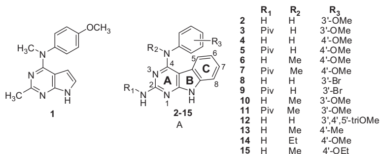
Figure 2. Parent pyrrolo[2,3- d ]pyrimidine 1 and target pyrimido[4,5- b ]indoles 2–15 .
