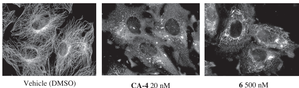
Figure 3. The effects of vehicle, CA-4 or 6 on interphase microtubules. A-10 cells were treated with vehicle, 20 nM CA-4 or 500 nM 6 . Following an 18 h incubation, the cells were fixed with cold methanol and microtubules were visualized by indirect immunofluorescence techniques with a β-tubulin antibody.
