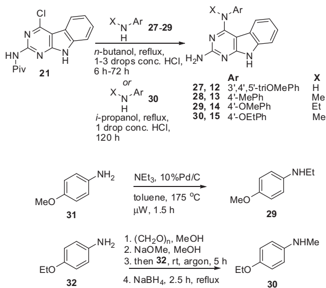
Scheme 2. Synthesis of compounds 12–15.
