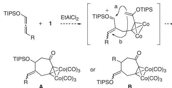
Scheme 2. Intermolecular [5 + 2] cycloaddition reaction of silyoxyallene and dicobalt acetylene complex 1 .
