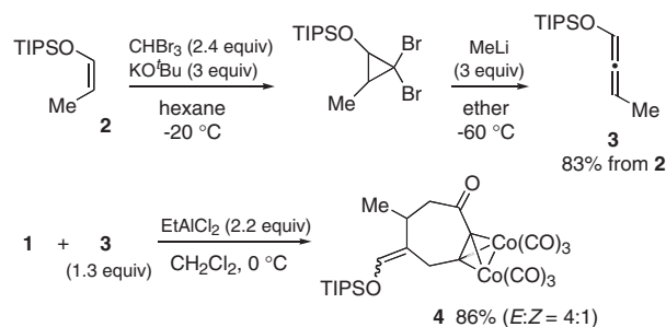
Scheme 3. Preparation and the [5 + 2] cycloaddition reaction of silyoxyallene 3 .
