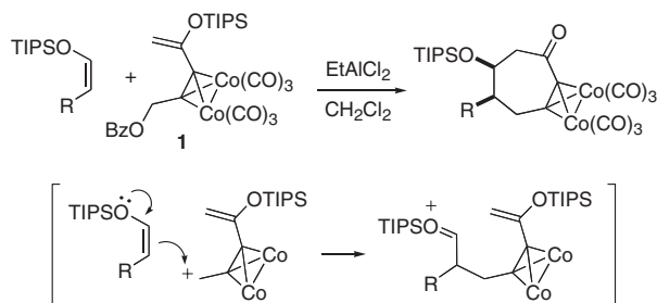
Scheme 1. Lewis acid-promoted intermolecular [5 + 2] cycloaddition reaction of dicobalt acetylene complex 1 (TIPSO: triisopropylsilyloxy).
