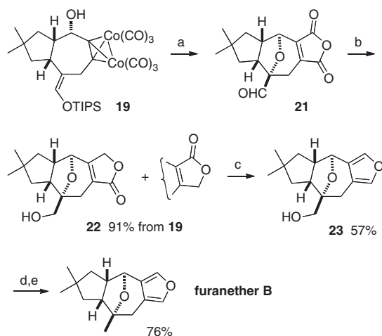
Scheme 7. Total synthesis of Furanether B. Reagents and conditions: (a) (NH 4 ) 2 Ce(NO 3 ) 6 (12 equiv), CH 3 CN–H 2 O, rt, 30 min; (b) NaBH 4 (5 equiv), THF–H 2 O, rt, 30 min then HCl (aq), rt, 30 min; (c) DIBAL (1.8 equiv), CH 2 Cl 2 , –78 °C, 10 min then HCl (aq); (d) Tf 2 O (1.5 equiv), 2,6-di- tert -butylpyridine (3 equiv), CH 2 Cl 2 –78 °C, 45 min; (e) LiBHEt 3 (2.1 equiv), THF, rt, 15 min.
