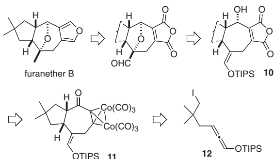
Scheme 5. Retrosynthetic analysis of furanether B.
