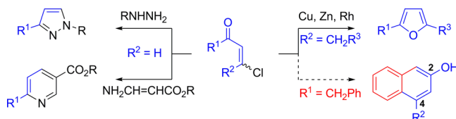
Scheme 1. Synthetic Utility of \beta -Chlorovinyl Ketones and Proposed Synthetic Route to 2-Naphthols
