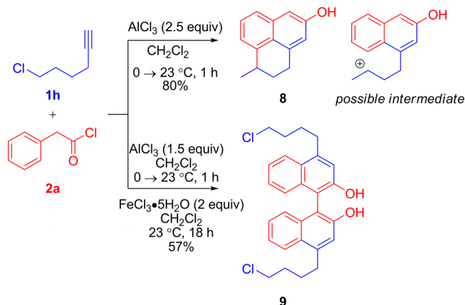
Scheme 4. Application to Other Aryl Compounds
