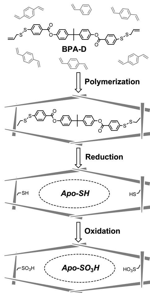
Scheme 2. Preparation of Holo-COOH
