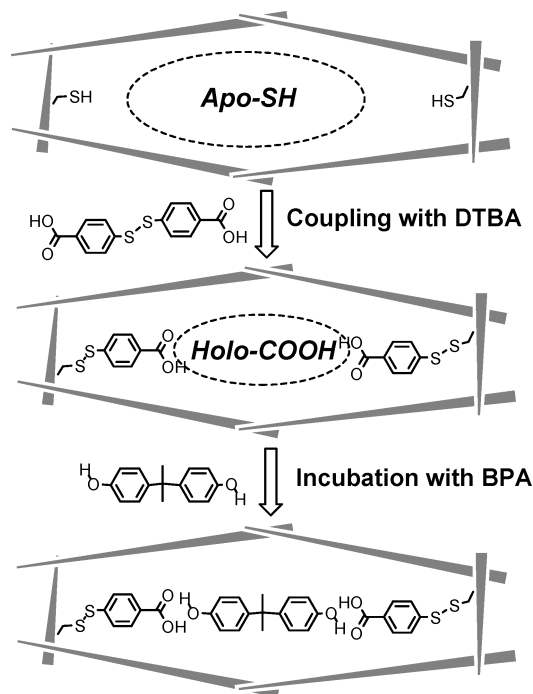
Scheme 2. Preparation of Holo-COOH
