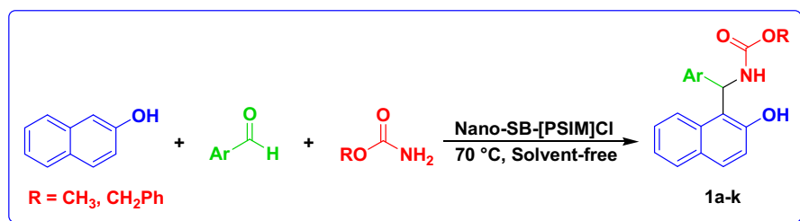
Scheme 2 The synthesis of \alpha -carbamatoalkyl- \beta -naphthols catalyzed by nano-SB-[PSIM]Cl
