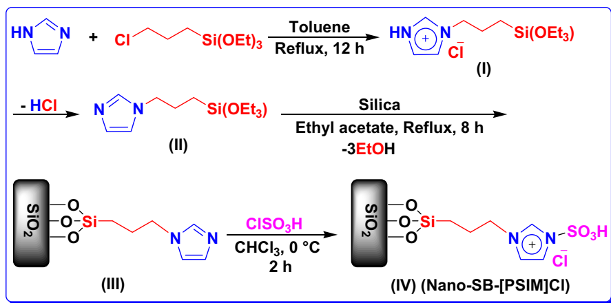
Scheme 1 The production of nano-SB-[PSIM]Cl
