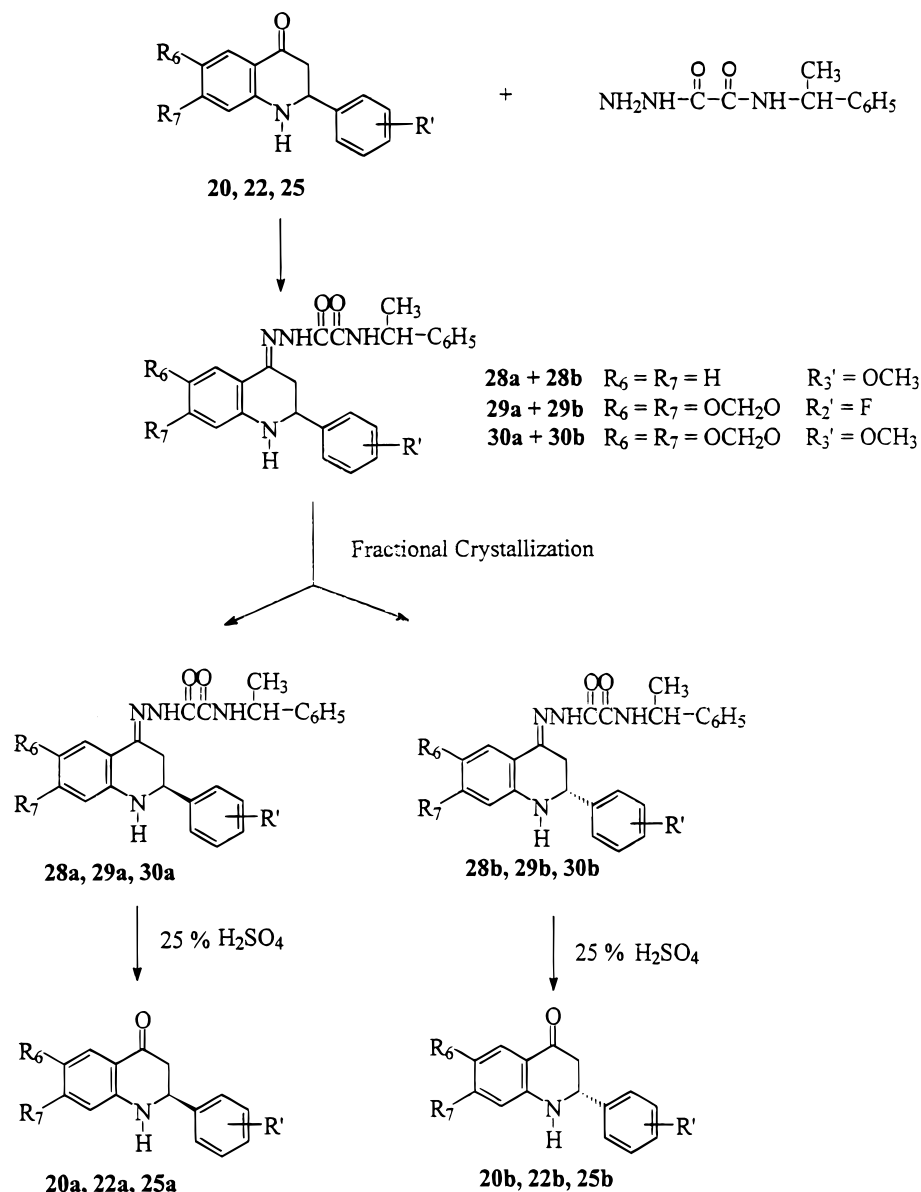
Scheme 3. Resolution of (±)-DHPQ Derivatives 20 , 22 , and 25 with (–)-5-(α-Phenethyl)semioxamazide
