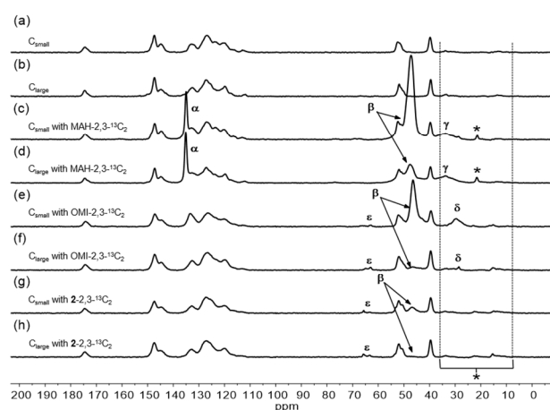
Figure 2. ^{13}\text{C} CP/MAS spectra of (a) C_{\text{small}} ; (b) C_{\text{large}} ; (c) C_{\text{small}} after reaction with MAH-2,3- ^{13}\text{C}_2 ; (d) C_{\text{large}} after reaction with MAH-2,3- ^{13}\text{C}_2 ; (e) C_{\text{small}} after reaction with OMI-2,3- ^{13}\text{C}_2 ; (f) C_{\text{large}} after reaction with OMI-2,3- ^{13}\text{C}_2 ; (g) C_{\text{small}} after reaction with 2-2,3- ^{13}\text{C}_2 ; (h) C_{\text{large}} after reaction with 2-2,3- ^{13}\text{C}_2 .
