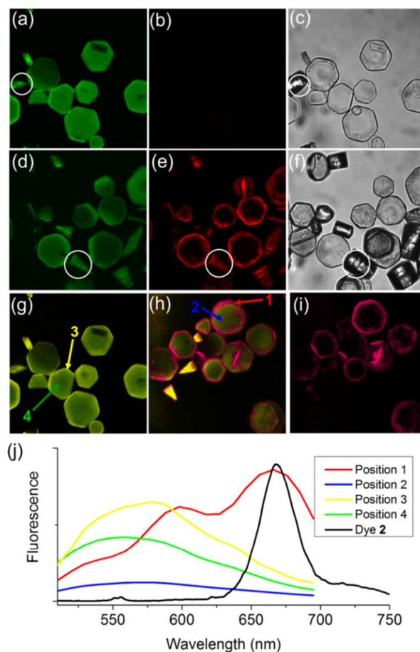
Figure 3. CLSM images of unmodified crystals excited at 488 nm (a) and at 633 nm (b). (c) Transmission image of unmodified crystal. CLSM images of modified crystals excited at 488 nm (d) and at 633 nm (e). (f) Transmission image of modified crystal. (g) Lambda scanning images (resolution: 9 nm) of unmodified crystals excited at 488 nm (g), and of BODIPY dye 2-modified crystals excited at 488 nm (h) and at 633 nm (i). (j) Uncorrected fluorescence spectra taken at the positions 1, 2, 3, 4 marked in (g) and (h) under CLSM conditions and of the BODIPY dye 2 in CH_2Cl_2 (excited at 488 nm).
