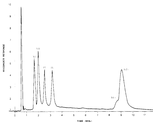
Figure 4. Gas chromatogram of a synthetic mixture of (I) the E and Z isomers of tetrachlorvinphos (950 pg), (III) 2,4,5-trichlorophenacyl chloride (52 pg), (IV) 2-chloro-1-(2,4,5-trichlorophenyl)ethanol (48 pg), (VI) 2,4,5-trichloroacetophenone (38 pg), and (VIII) 1-(2,4,5-trichlorophenyl)ethanol (42 pg). GC conditions: glass column 1.83 m \times 4 mm i.d. packed with 3% SE-30 on Chromosorb WHP; injector, column, and detector temperatures, 175, 170, and 295 °C, respectively; 63 Ni ECD; carrier gas (nitrogen) flow rate, 40 mL/min.
