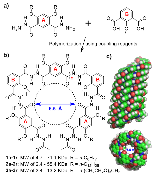
Figure 1. a) Structures of building blocks A and B used to produce nanotubes 1-3 . b) Foldamer-based approach for constructing H-bonded pore-forming polymeric anion channels 1-3 , having a hollow cavity of 6.5 Å in diameter after excluding van der Waals volume of atoms decorating channel's interior. c) Side and top views of a helically folded polymer nanotube computationally optimized in POPC membrane (Supporting Information).
