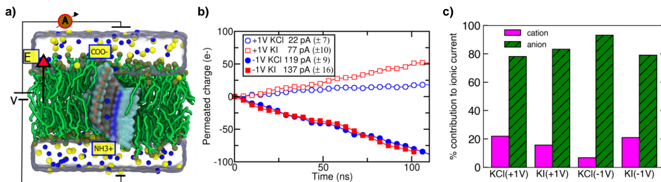
Figure 4: Ionic-current through the HP24 channel simulated using the all-atom MD method. a) A cut-away view of the simulation system where the channel is shown as a molecular surface coloured according to the local atom types: red (oxygen), blue (nitrogen) and cyan (carbon). The yellow labels specify the location of the terminal groups of the channels. Nitrogen atoms of the lipid head groups are shown as tan sphere whereas the tails of the lipid molecules are shown as thick green lines. K + (yellow) and Cl - (blue) ions (at 1 M concentration) are shown as spheres whereas the volume occupied by water is represented by a semi-transparent surface. b) The total permeated charge (integrated ionic current) as a function of the simulation time in the units of the elementary charge, e. The slope of each line gives the average current. The inset specified the average current values with the error bars for each system. c) Percentage of total current carried by the cation and anion species in the simulations of the KCl and KI systems.
