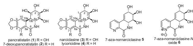
Figure 1. Amaryllidaceae alkaloids and aza-nornarciclasine.
