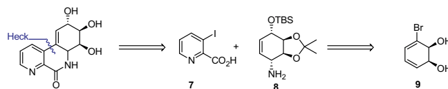
Figure 2. Retrosynthetic plan for aza-nornarciclasine analogues.
