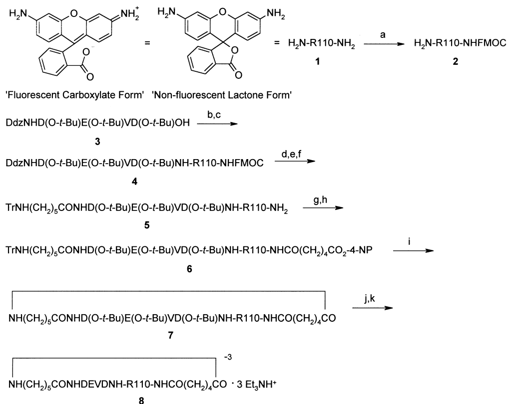
Scheme 1. Reagents and conditions: (a) Fmoc chloride, DIEA, DMF, rt; (b) IBCF, NMM, THF, -10^{\circ}\text{C} ; (c) 2 , THF, -10^{\circ}\text{C} to rt; (d) 2.5% TFA in CH 2 Cl 2 followed by NMM, rt; (e) mixed anhydride of TrNH(CH 2 ) 5 COOH in THF, 6 rt; (f) 2% piperidine in DMF, rt; (g) adipoyl chloride, collidine, THF, rt; (h) 4-nitrophenol, THF, rt; (i) 5% TFA in CH 2 Cl 2 followed by CH 2 Cl 2 and DIEA, rt; (j) 25% TFA in CH 2 Cl 2 , rt; (k) Et 3 N, MeOH, rt
