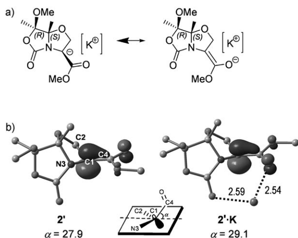
Figure 3. a) Structure of enolate 2' showing the greater contribution of the carbanionic resonance form. b) Minimum-energy structures and HOMO of “naked” ( 2' ) and potassium ( 2'·K ) enolates, calculated at the B3LYP/6-31+G(d) level of theory. Distances are given in Å and angle \alpha in degrees.
