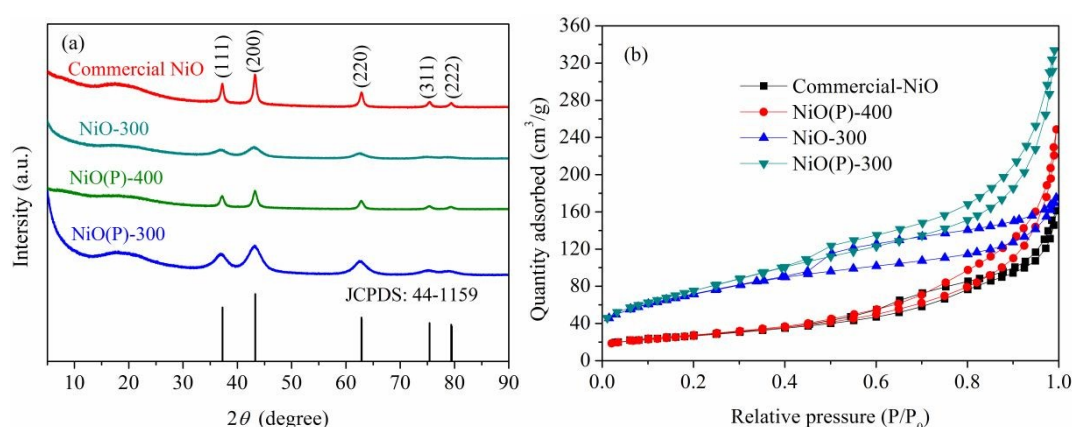
Figure 1 (a) XRD patterns and (b) N_2 adsorption-desorption isotherms of the as-prepared catalysts and NiO nanoparticles.
