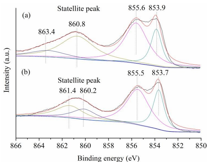
Figure 3 XPS spectra of Ni 2p 3/2 of (a) NiO(P)-300 and (b) commercial NiO samples.
