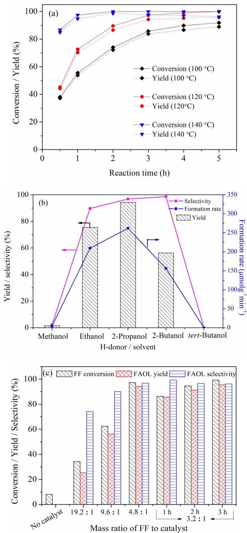
Figure 4 (a) Effect of reaction temperature and reaction time on CTH of FF to FAOL
