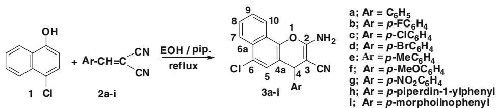
Scheme 1 Synthesis of 4 H -benzo[ h ]chromene-3-carbonitrile derivatives ( 3a–i )
