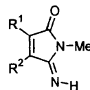
7 R 1 = Me, R 2 = H 8 R 1 = H, R 2 = Me
