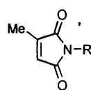
1 R = CH 2 Ph 2 R = Ph
