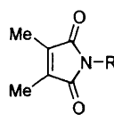
13 R = Ph 14 R = CH 2 Ph
