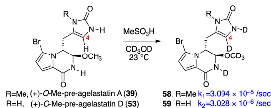
Scheme 14. Rate Constants for the Deuterium Incorporation at C4 of (+)-39 and (+)-53
