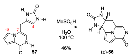
Scheme 13. Formation of the C4–C13 Bond upon Acidic Treatment of Enamide 57
