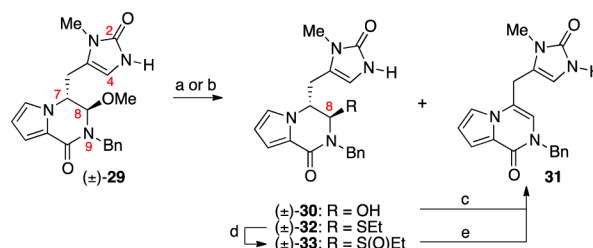
Scheme 6. Formation of Pyrrolopyrazinone 31 under Various Conditions a
