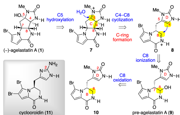
Scheme 1. Retrosynthetic Analysis of (-)-Agelastatin A (1)
