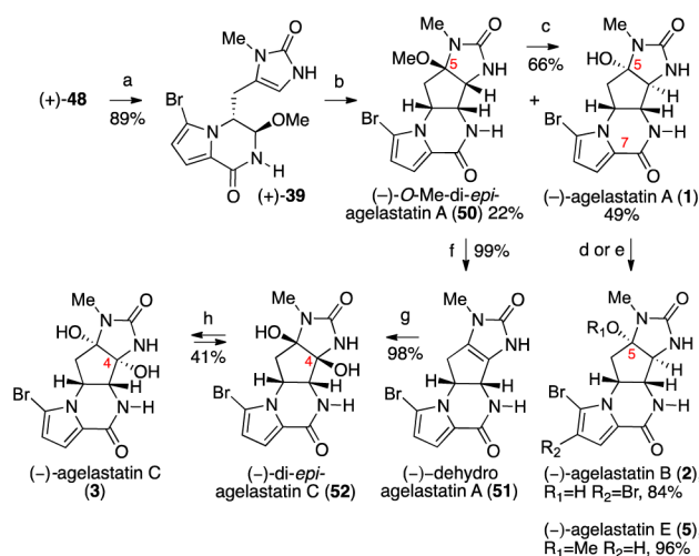
Scheme 11. Enantioselective Synthesis of (–)-Agelastatins A–C (1–3) and E (5) a
