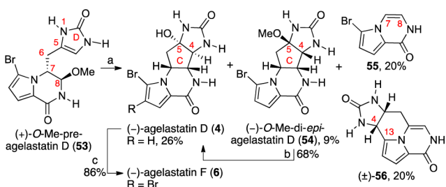
Scheme 12. Total Synthesis of (–)-Agelastatin D (4) and the Formation of Byproducts 55 and 56 a
