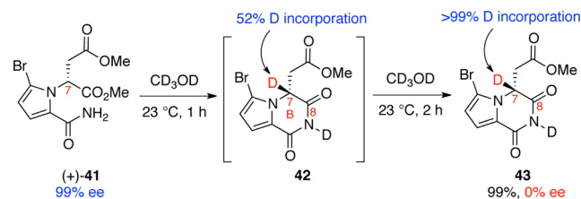
Scheme 9. Cyclization and Deuterium Incorporation at C7 of Amide (+)-41
