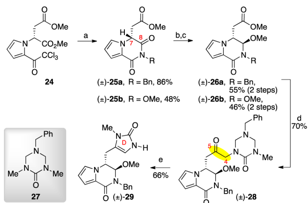
Scheme 5. Synthesis of Imidazolone (±)-29 a
