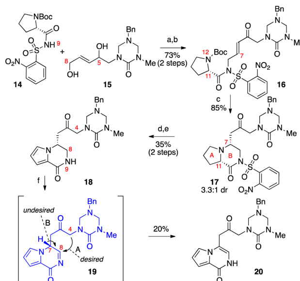
Scheme 3. Synthesis of Key Bicyclic 18 and Attempted Oxidation–Cyclization a
