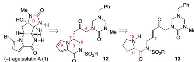
Scheme 2. Early Approach toward (-)-Agelastatin A (1)
