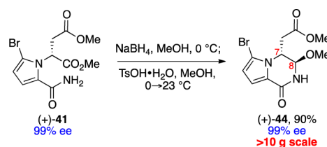
Scheme 10. Synthesis of Bicycle (+)-44
