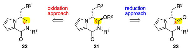
Scheme 4. Two Strategies for the Introduction of the C8-Hemiaminal Ether 21
