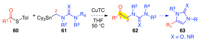
Scheme 15. Versatile Synthesis of Azaheterocycle 63
