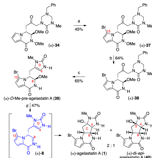
Scheme 8. Our First-Generation Total Synthesis of ( \pm )-Agelastatin A (1) a
