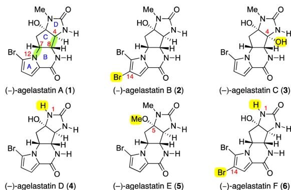
Figure 1. Structures of (–)-agelastatins A–F (1–6).
