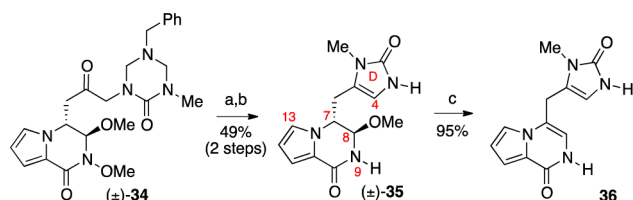
Scheme 7. Synthesis of Imidazolone Derivative ( \pm )-35 and Its Reactivity under Acidic Conditions a
