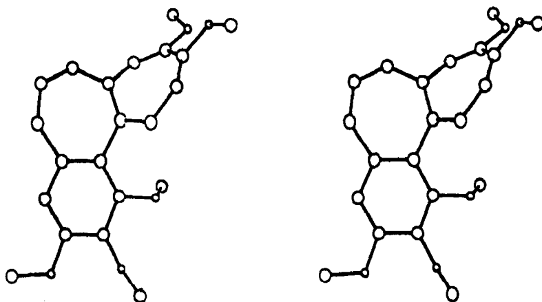
Fig. 3. Stereoscopic view of the X-ray crystal structure of 1,2,3,9,10-pentamethoxybenzo[a]heptalene (9). Only the C- and O-atoms are shown. The (7aP)-configuration of the heptalene skeleton is displayed.
