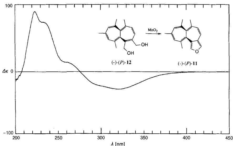
Fig. 6. CD Spectrum (EtOH) of (-)-(P) -6,7,9,11-tetramethylhepteno[1,2- c ]furan (-)-(P) -11 [42]
