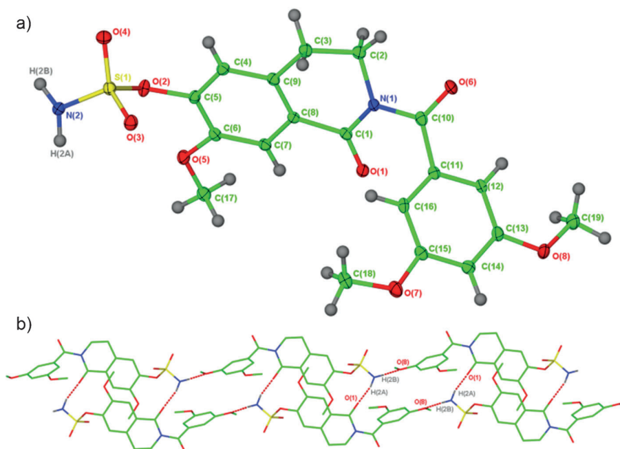
Figure 3. a) Single-crystal X-ray structure of 17f . Ellipsoids are depicted at 30% probability. b) Part of the crystal lattice packing diagram of 17f to illustrate the hydrogen-bonded linear arrangements present in the gross structure.
