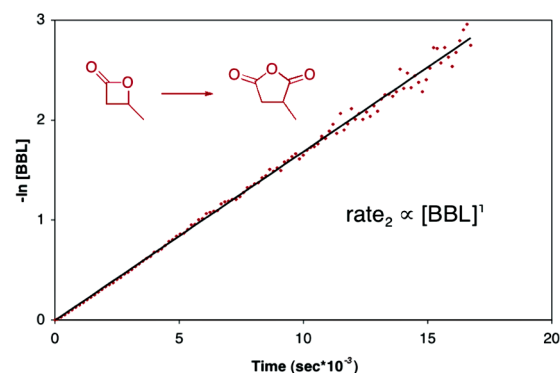
Figure 7. Plot of -\ln[\text{BBL}] versus time for the carbonylation of BBL to MSA. Reaction performed in 1,4-dioxane and monitored with in situ IR spectroscopy ( \nu_{\text{C=O}} BBL = 1827 \text{cm}^{-1} ). [\text{I}] = 4.0 \text{ mM} , [\text{BBL}]_0 = 1 \text{ M} , P_{\text{CO}} = 850 \text{ psi} , T = 40^\circ \text{C} .
