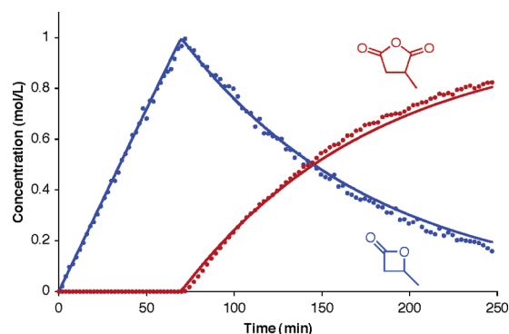
Figure 8. Comparison of simulated (solid lines) with experimental data (points, same as Figure 3) for the double carbonylation of PO in 1,4-dioxane. [PO]_0 = 1.0 M, [I] = 4.0 mM, P_{CO} = 850 psi, T = 40 °C.
