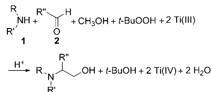
Scheme 2. Synthesis of 1,2-Amino Alcohols Mediated by the \text{TiCl}_3 / t -BuOOH System
