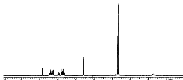
Figure 3. ^1\text{H} NMR spectrum (200 MHz, \text{CDCl}_3 ) of compound 11 .
