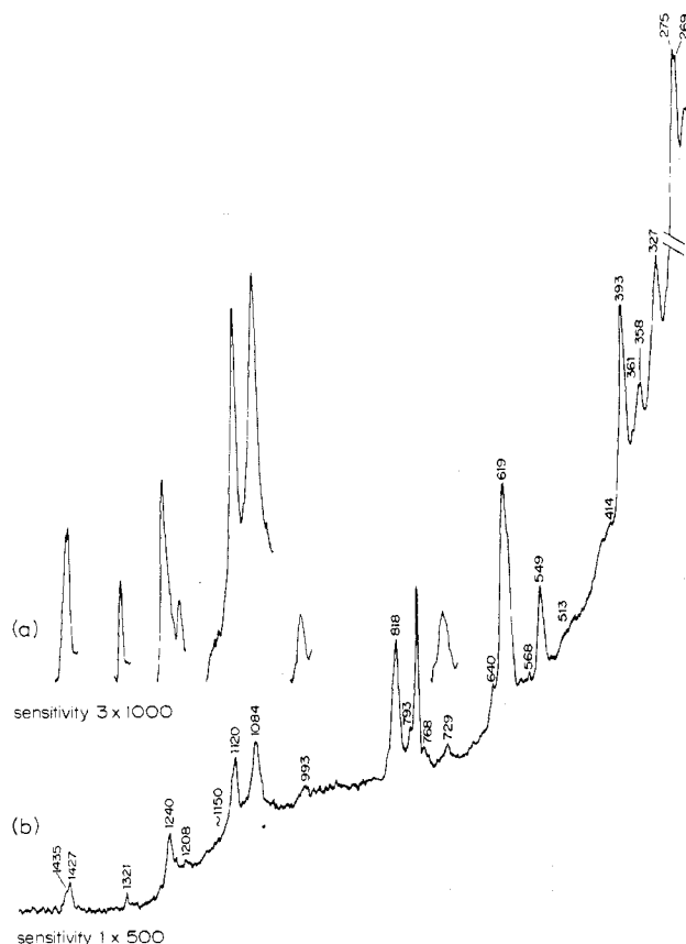
Figure 1. Raman spectrum of \text{I}(\text{OSO}_2\text{CF}_3)_3 .
