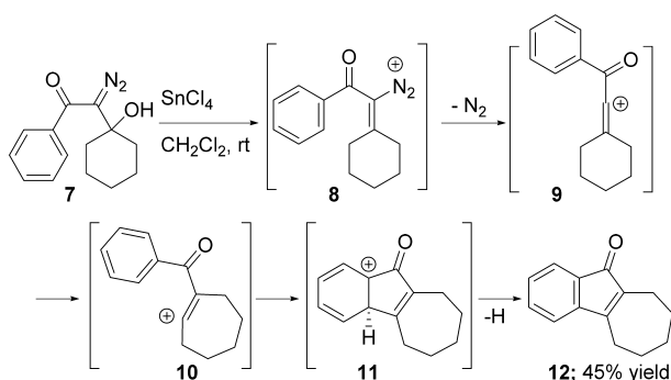
Scheme 2. Indenone Formation via Aromatic Vinylation of a Vinyl Cation
