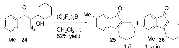
Scheme 5. Meta Substitution Leads to a Mixture of Regioisomers
