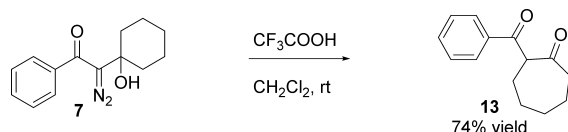
Scheme 3. TFA Mediated Ring Expansion
