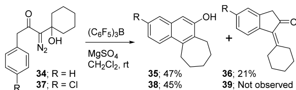
Scheme 8. Change in Tether Length Provides 2-Naphthol Product
