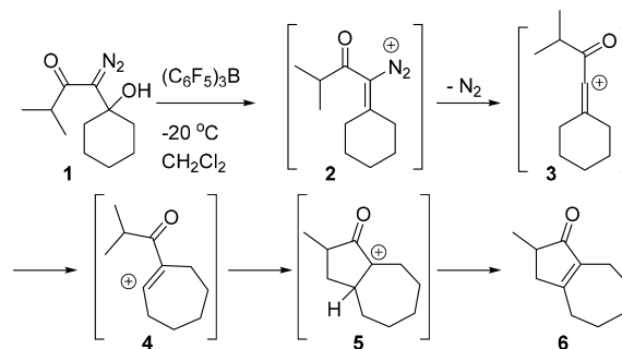
Scheme 1. Use of \beta -Hydroxy- \alpha -diazo Ketone in a C–H Insertion Reaction
