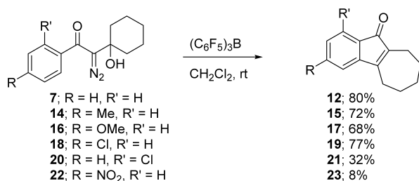
Scheme 4. Inden-1-one Formation by Intramolecular Vinylation of Aryl Rings
