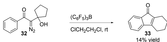
Scheme 7. Formation of 1,2,3,4-Tetrahydro-9H-fluoren-9-one
