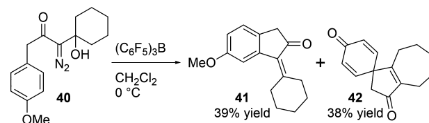
Scheme 9. Spirocycle Formation
