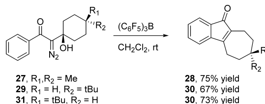
Scheme 6. Effect of Substitution on Aliphatic Ring
