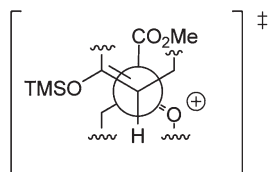
Figure 1. Proposed transition state for the formation of 14 .
