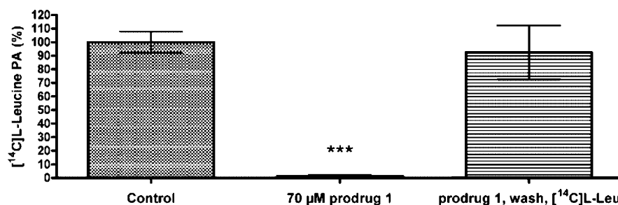
Figure 2. Mechanism of prodrug 1 rat brain uptake. The PA product of 0.2 \mu\text{Ci/mL} [ ^{14}\text{C} ]-L-leucine in the absence or presence of 1 . The control PA product 0.02059 \pm 0.00323 mL/s/g (mean \pm SD, n = 5 ) is decreased to 0.000317 \pm 0.000136 mL/s/g (mean \pm SD, n = 3 ) in the presence of 70 \mu\text{M} 1 (98.5% inhibition). The uptake of [ ^{14}\text{C} ]-L-leucine is recovered after washing the prodrug from the brain capillaries, demonstrating the PA product of 0.01902 mL/s/g. An asterisk denotes a statistically significant difference from the respective control (*** P < 0.001 , one-way ANOVA, followed by Dunnett's t test).
