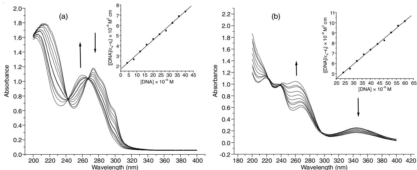
Fig. 6. (a) Electronic absorption titration of complex 1 ( 5 \times 10^{-4} \text{ M} ) with ct-DNA (0-100 \mu\text{M} ) in Tris-buffer ( \text{pH} = 7.2 ); Inset: plot of [\text{DNA}]/(\epsilon_a - \epsilon_f) versus [\text{DNA}] . (b) Electronic absorption titration of complex 2 ( 5 \times 10^{-4} \text{ M} ) with ct-DNA (0-100 \mu\text{M} ) in Tris-buffer ( \text{pH} = 7.2 ); Inset: plot of [\text{DNA}]/(\epsilon_a - \epsilon_f) versus [\text{DNA}]
