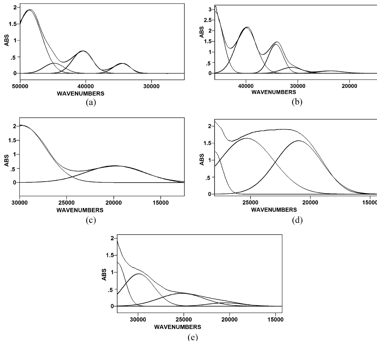
Figure 6. Deconvoluted electronic spectra of (a) 6.72 \times 10^{-4} M DHB − at room temperature in pH 6.2 phosphate buffer having a path length of 0.1 cm; (b) 2.33 \times 10^{-4} M 2 at room temperature in pH 5 aqueous solution having a path length of 1.0 cm; (c) 6.57 \times 10^{-4} M 2 at room temperature in pH 10 aqueous solution having a path length of 1.0 cm; (d) a polarized spectrum of 3 at room temperature (3.783 M, pure single crystal, 0.013 mm thick) with the electric vector parallel to c ; and (e) same as (d), but with the electric vector parallel to b .
