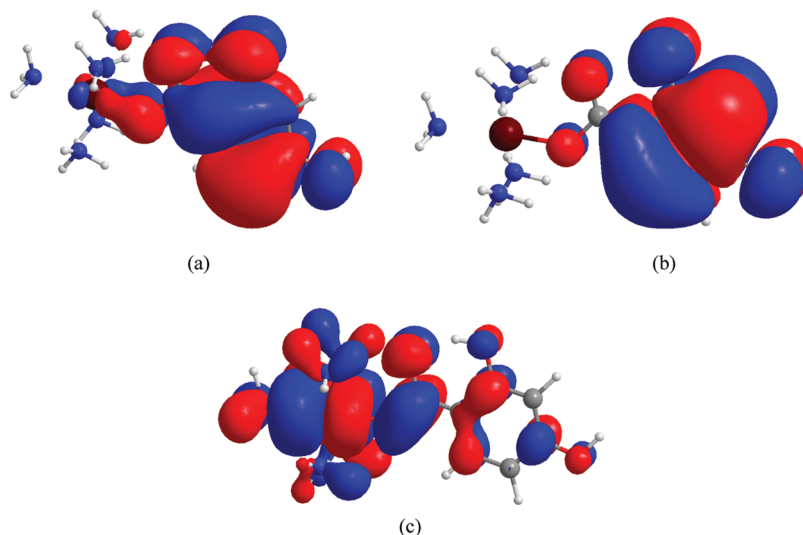
Figure 7. Contour plots of principal orbitals involved in the DHB − (π) → Ru[d(π)] LMCT transitions in 2 . The same isocontour value applies to all three plots. (a) HOMO β spin-orbital, a DHB − (π)-donor orbital; (b) HOMO-1 β spin-orbital, a second DHB − (π)-donor orbital; and (c) LUMO β spin-orbital, a Ru[d(π)] acceptor orbital. The transition amplitudes for the elementary excitations HOMO β → LUMO β and HOMO-1 β → LUMO β are very large and dominate the overall intensities of the two low-lying ligand-to-metal charge-transfer transitions in 2 (Table 3).
