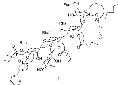
Fig. 4. Key HMBC Correlations from H to C for Compound 1
