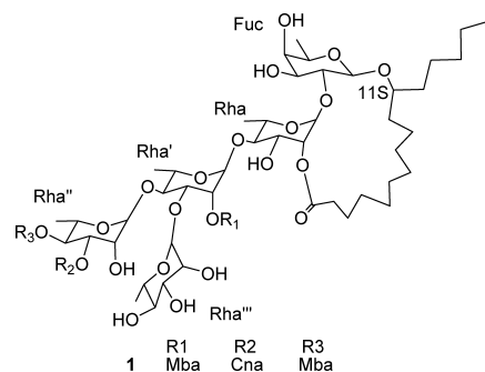
Fig. 1. Structure of Batatoside III ( 1 )
