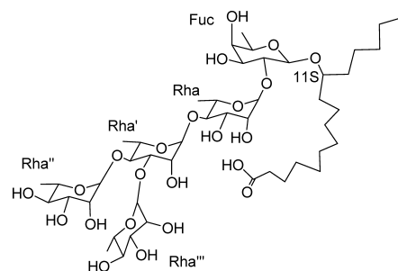
Fig. 3. Structure of Simonic Acid B ( 4 )
