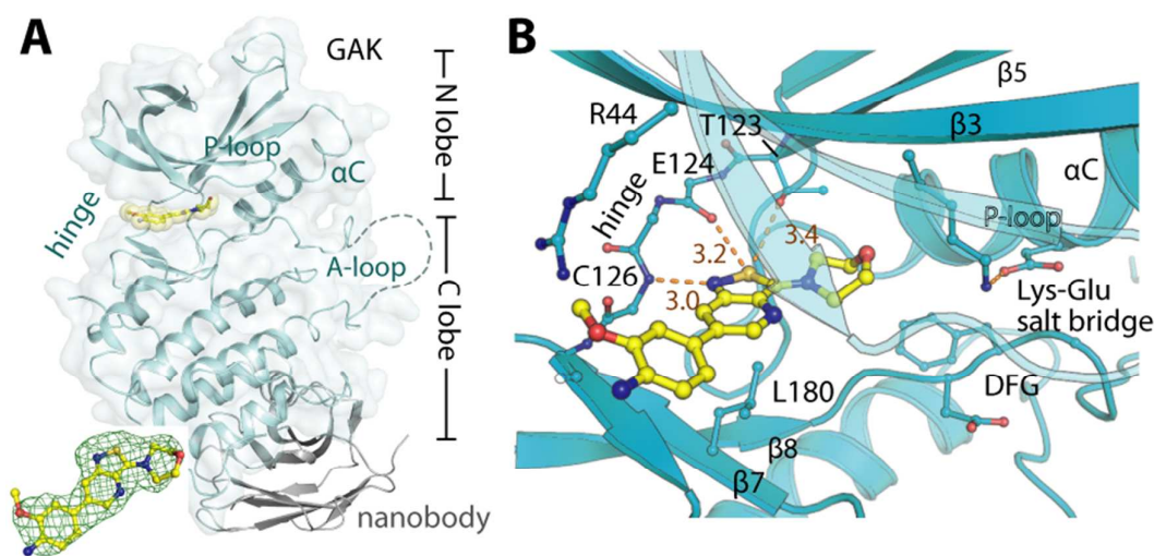
Figure 3 : Structure of GAK in complex with 12i . A ) Overview of GAK:NbGAK_4 complex with inhibitor 12i bound. The inset shows |F_o| - |F_c| omitted map contoured at 3\sigma for the bound inhibitor. B ) Detailed interactions of 12i within the GAK ATP binding site.
