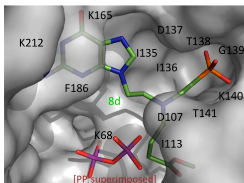
Figure 6. The docking of 8d containing a -\text{COOMe} attachment to the active site of HGPRT. The location of \text{PP}_i when it binds in the enzyme has been superimposed from the structure of human HGPRT in complex with immucillinHP, \text{PP}_i , and \text{Mg}^{2+} .
