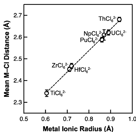
Figure 4. Plot of the mean M–Cl bond distances (Å) in (\text{Ph}_4\text{P})_2\text{MCl}_6 ( \text{M} = \text{Ti}, \text{Zr}, \text{Hf}, \text{Th}, \text{U}, \text{Np}, \text{Pu} ) relative to the ionic radius of \text{M} . 70 A linear fit to the data (dashed line) gives the equation y = (1.75 \pm 0.02 \text{ Å}) + (0.98 \pm 0.02)x . Error bars are taken from the standard deviation in the mean distance of crystallographically inequivalent M–Cl bonds.
