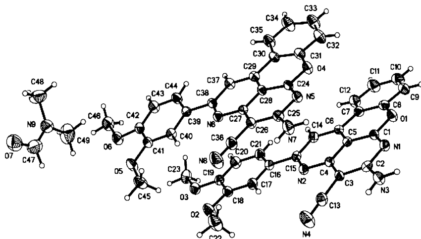
Scheme 1. Possible Mechanism for the Formation of the Product
