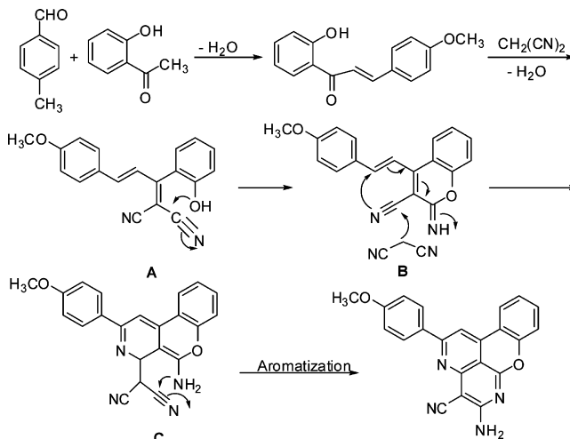
Scheme 1. Possible Mechanism for the Formation of the Product
