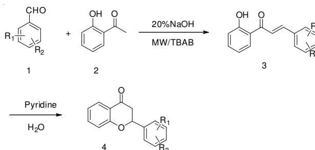
Scheme-I: Synthesis of enantiomers 2-phenychroman-4-ones
