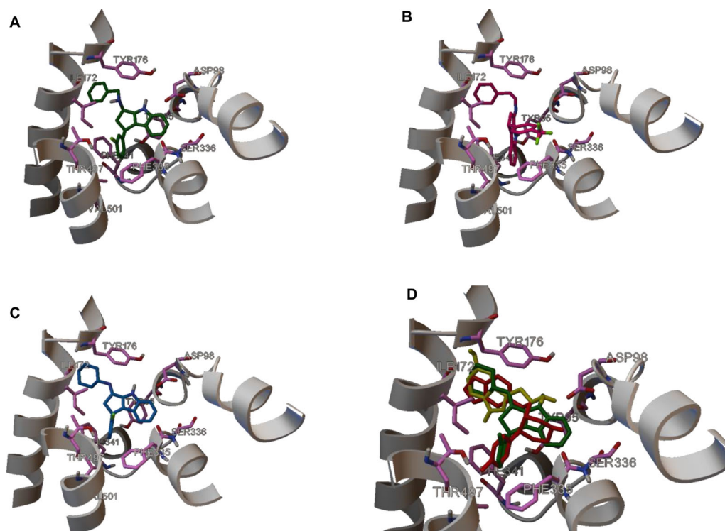
Figure 2. Binding modes on TS3 transporter active site a) amine 3cc (1R, 3R), b) imine 4aba (R), c) imine 4acb (R) d) binding comparison of 4acb (R) (green), paroxetine (red) and serotonin (yellow).
